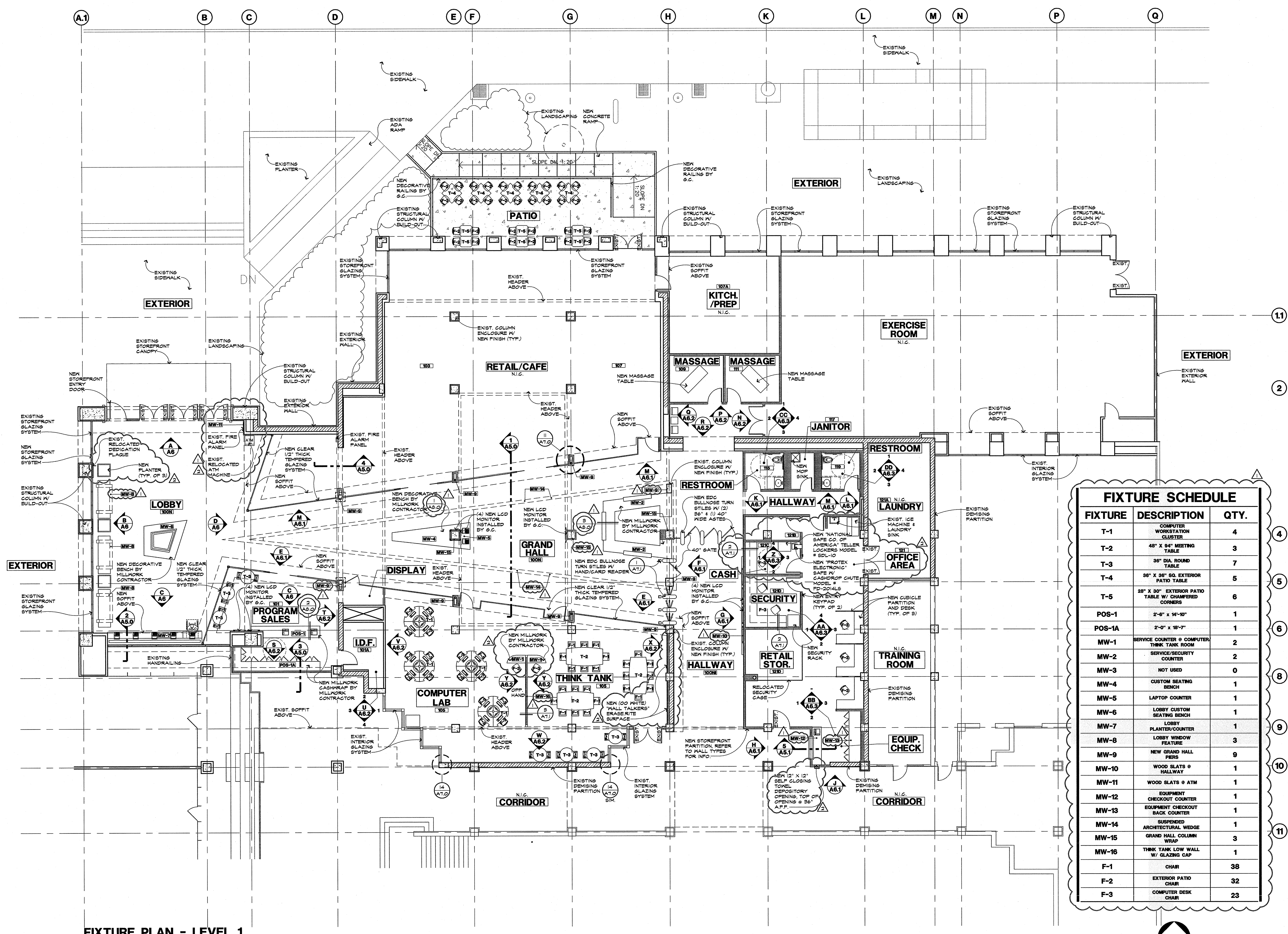
FIXTURE PLAN - LEVEL 1
